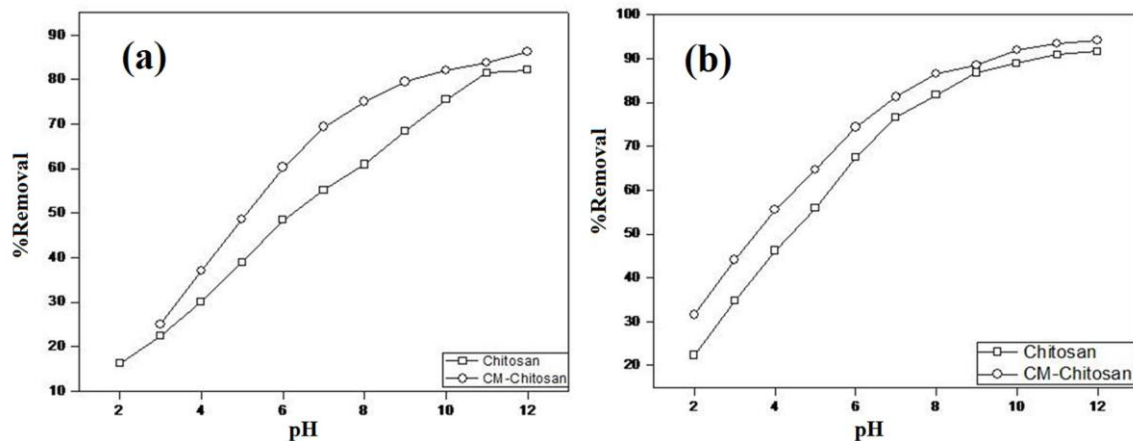
Fig. 6: Effect of pH on the adsorption of (a) \text{Cu}^{+2} and (b) \text{Pb}^{+2} by Chitosan and CM-Chitosan.
