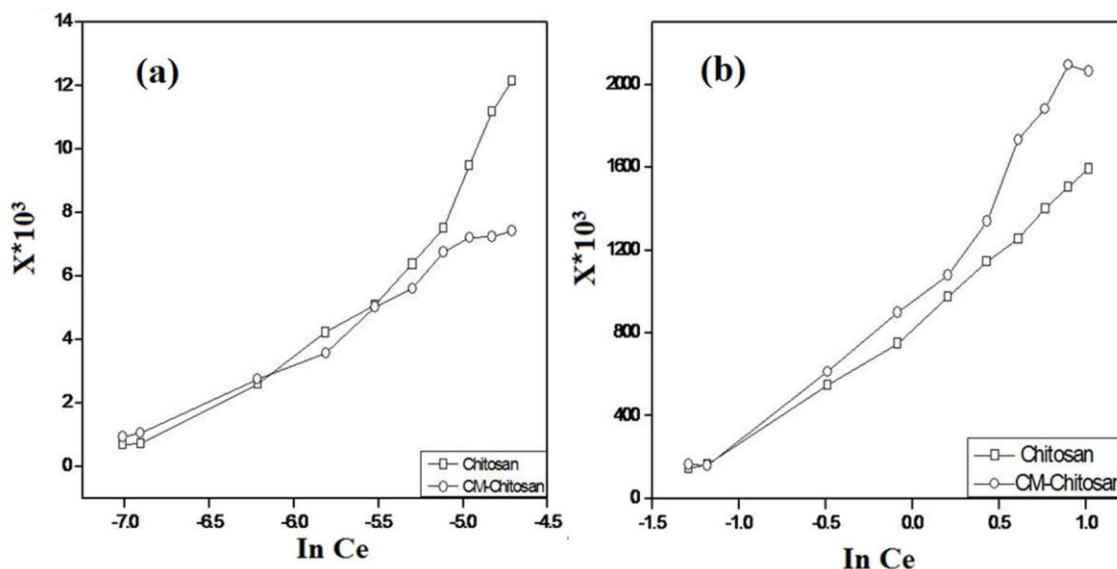
Fig. 10: Temkin isotherm for adsorption of (a) Cu 2+ and (b) Pb 2+ .
