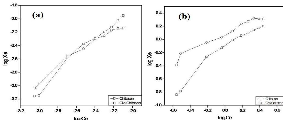
Fig. 9: Freundlich isotherm for (a) Cu 2+ and (b) Pb 2+
