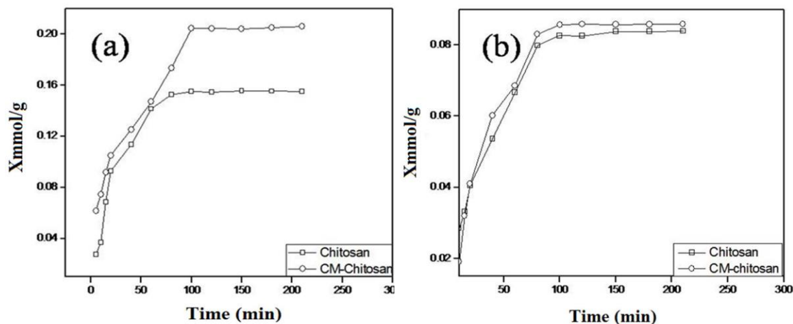
Fig. 7: Time study of adsorption of (a) \text{Cu}^{+2} and (b) \text{Pb}^{+2} by Chitosan and CM-Chitosan.
