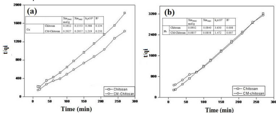
Fig. 8: Pseudo 2 nd order kinetics for (a) Cu 2+ and (b) Pb 2+ .
